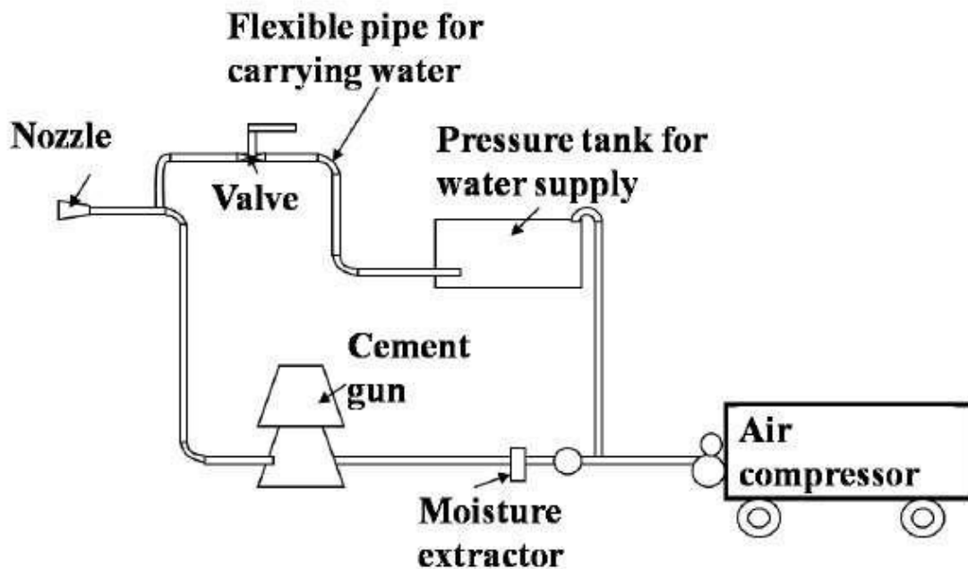
FIG-16 SHOTCRETE
