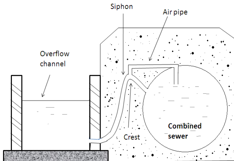
Siphon spillway Figure 13.15
