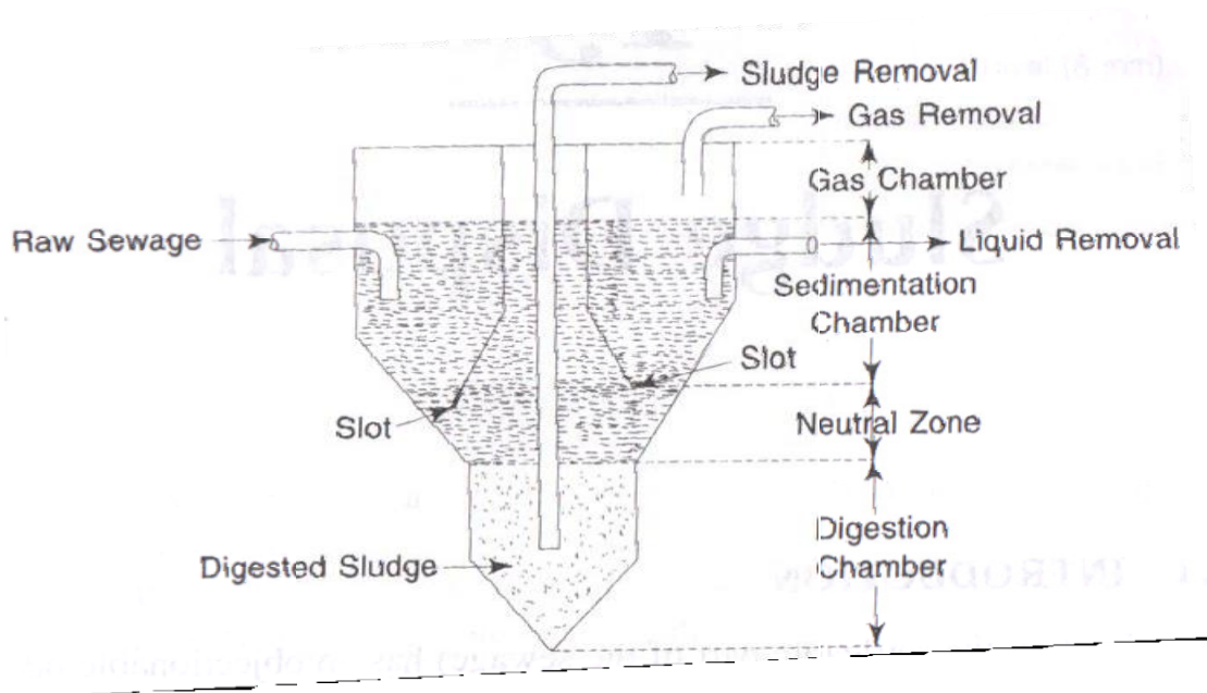
IMHOFF TANK
