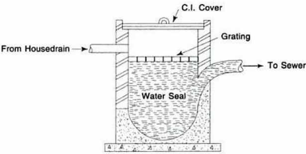
Gully Trap Fig. 17.7
