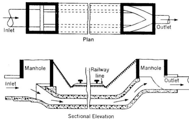
Inverted Syphon
