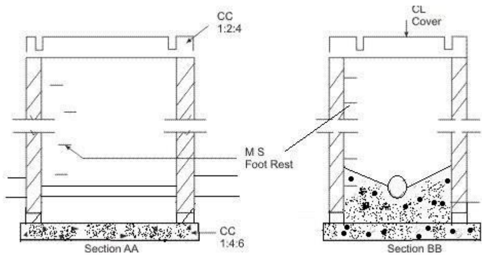
Shallow Manhole Figure 13.1
