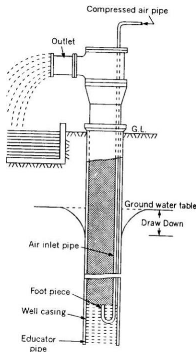
Air lift pump Figure 13.17
