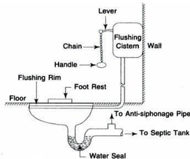
Water Closet Fig.17. 5
