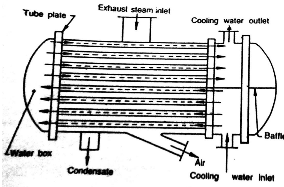
Fig. 6.5 Surface Condensers
