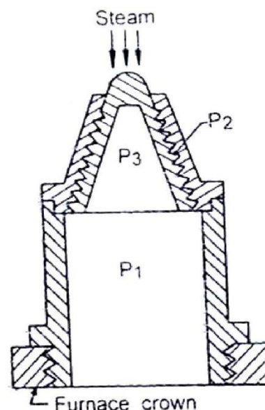
Fig. 3.12 Fusible plug
