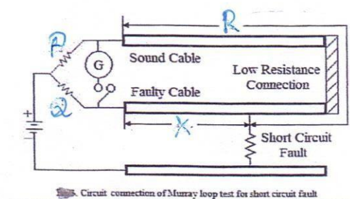
Fig. 5. Circuit connection of Murray loop test for short circuit fault
