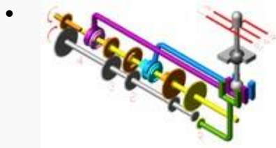
Neutral (blue and purple in the middle, green disengaged)
